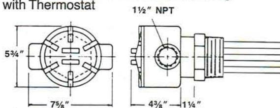
NEMA 4/7 Explosion Resistant Housing with Thermostat
