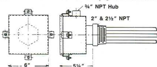
NEMA 4 Moisture Resistant Housing with Thermostat
