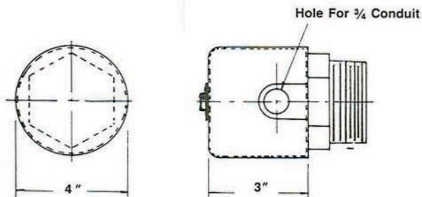
NEMA I with Thermostat
