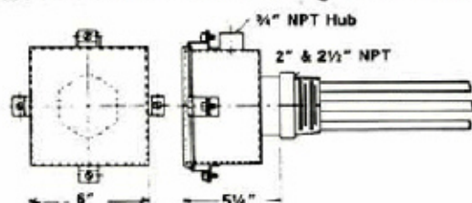
NEMA 4 Moisture Resistant Housing with Thermostat
