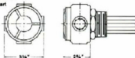
NEMA 4/7 Explosion Resistant Housing with Thermostat
