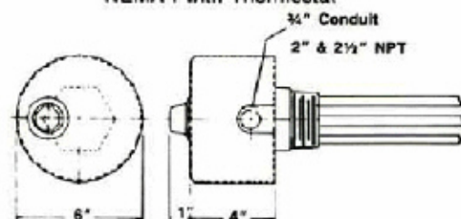
NEMA 1 with Thermostat
