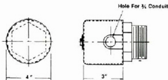
NEMA I with Thermostat
